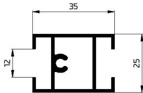
22109 SASH 575.26 GR/M W.T-14mm
