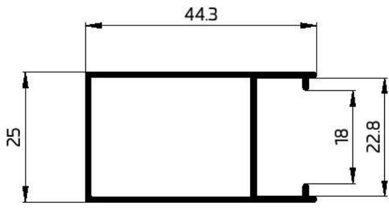
22041 SLIDING SASH 388.79 GR/M W.T-1mm
