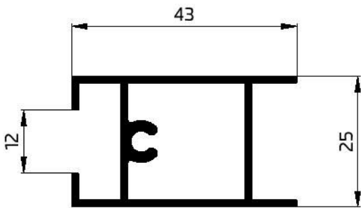
22108 SLIDING RAIL SASH 63188 GR/M W.T-14mm
