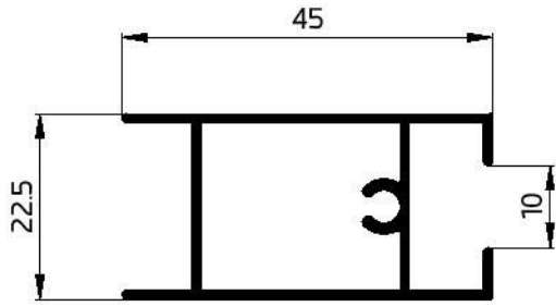
22024 SLIDING RAIL SASH 412.00 GR/M W.T-1.1mm
