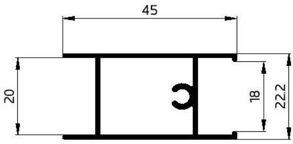
22039 SLIDING RAIL SASH 439.65 GR/M W.T-1mm
