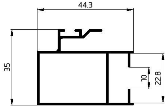
22025 SLIDING INTERLOCK 480 GR/M W.T-1.1mm
