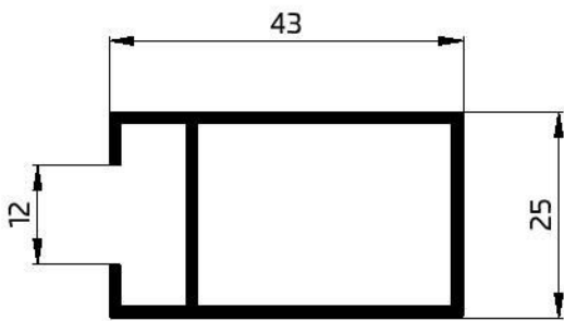
22115 SLIDING SASH 53103 GR/M W.T-14 mm
