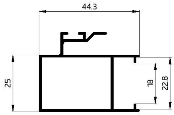
22040 SLIDING INTERLOCK SASH 525.66 GR/M W.T-1mm
