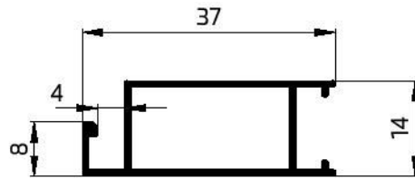
22030 FLY SCREEN 246.01 GR/M W.T-1mm
