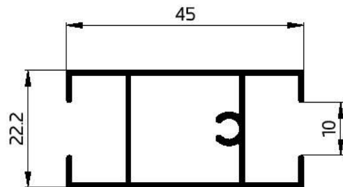
22027 SLIDING DIVISOR 438.11 GR/M W.T-1mm
