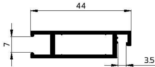
22113 FLY SCREEN 460.08 GR/M W.T-2 mm
