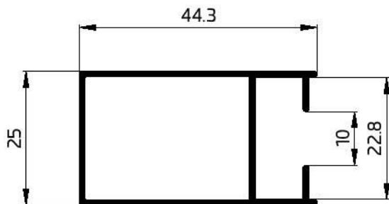
22026 SLIDING SASH 380 GR/M W.T-1mm
