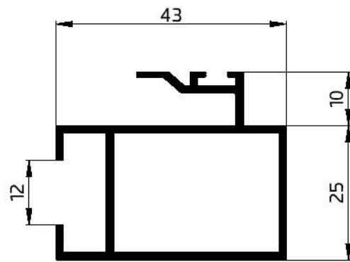
22114 SLIDING INTERLOCK 655.29 GR/M W.T-14 mm
