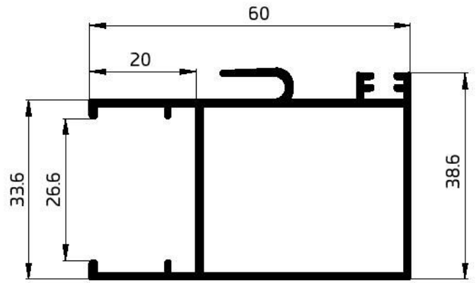
22089 INTERLOCK SASH 728 GR/M T-12mm
