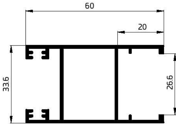
22088 SIDE SASH 728 GR/M T-12mm
