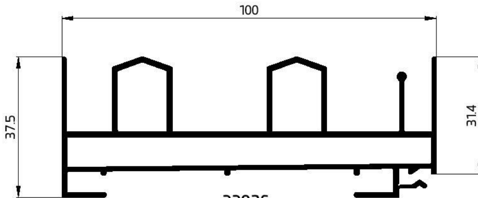
22036 SLIDING TUBULAR FRAME 100 1,501.63 GR/M T-1.4mm
