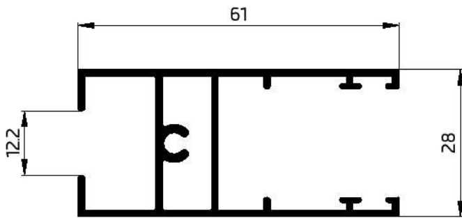
22023 RAIL SASH S.GLASS 779.81 GR/M W.T-13mm
