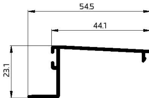
22034 BEAD FOR FIXED GLASS 275.79 GR/M T-1.15mm
