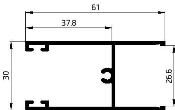
22090 RAIL SASH 588 GR/M T-12mm
