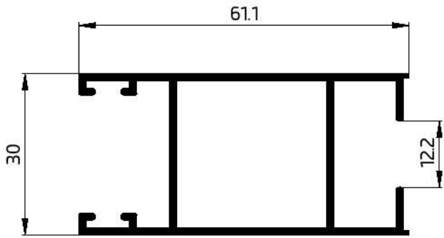
22021 SIDE SASH FOR 22023 734.80 GR/M W.T-13mm
