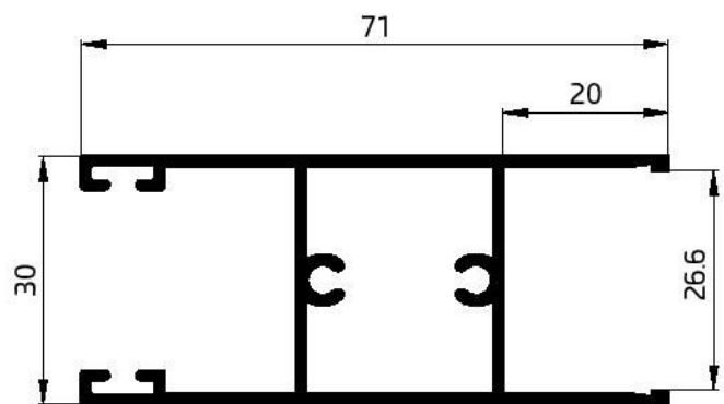
22092 TOP SASH 770 GR/M T-12mm
