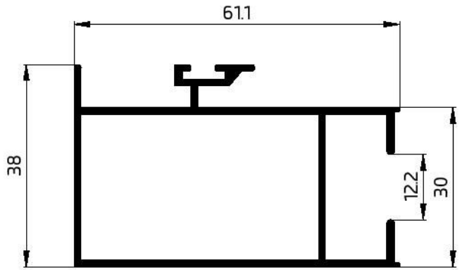
22022 INTERLOCK SASH FOR 22023 803.33 GR/M W.T-13mm
