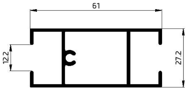
22031 DIVISOR SASH S.GLASS 753.68 GR/M W.T-13mm
