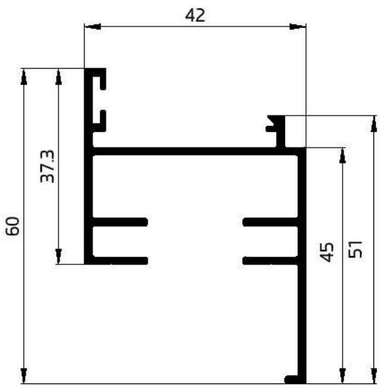
31019 HINGE FRAME 42 738.63 GR/M W.T-1.5mm
