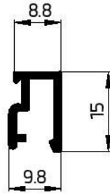
31043 BEAD 27 139.31 GR/M W.T-125mm
