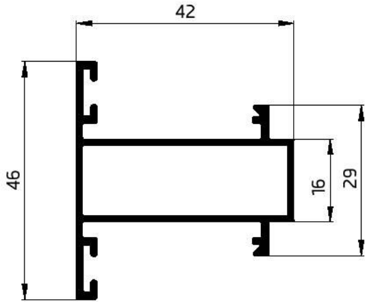
31059 T-SECTION 42X16 614.62 GR/M W.T = 12 mm
