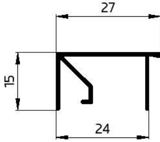
31003 BEAD 27 178.51GR/M W.T-0.9mm
