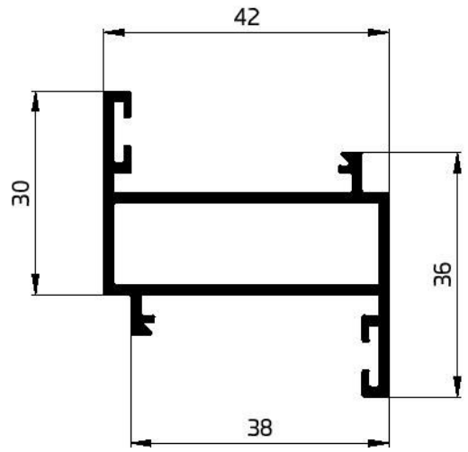
31041 HINGED SASH 42 696.22 GR/M W.T-15mm
