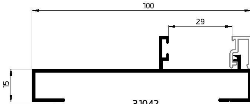
31042 HINGE FRAME 100 740 GR/M W.T-15mm
