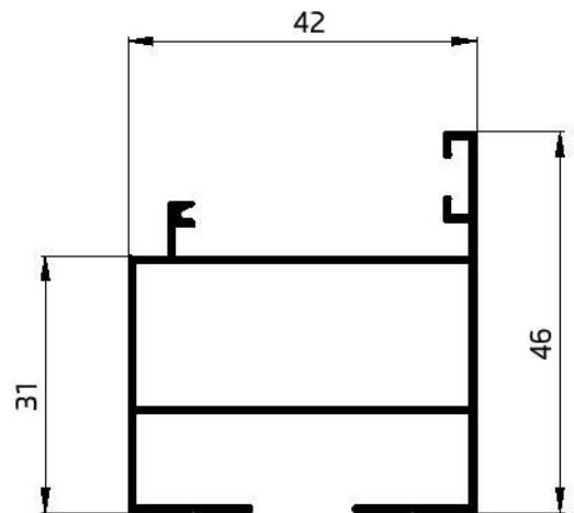
31080 HINGE SASH 42 500 GR/M W.T = 0.9 mm
