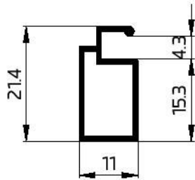
31001 FLY SCREEN 157.25 GR/M W.T-0.9mm
