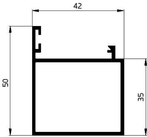
31038 HINGED FRAME 42 728.89 GR/M W.T-15mm
