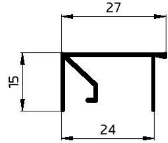
31013 BEAD 27 168.7 GR/M W.T-0.85mm
