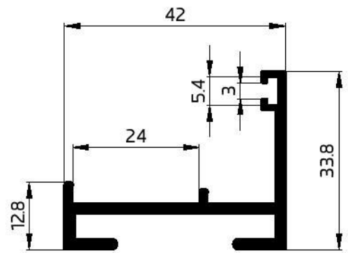
52000 CW-FRAME 559.91 GR/M WT-2.0 mm
