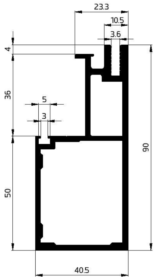
55504 CW-END PROFILE 40.5X50 1922.67 GR/M WT-2.5 mm
