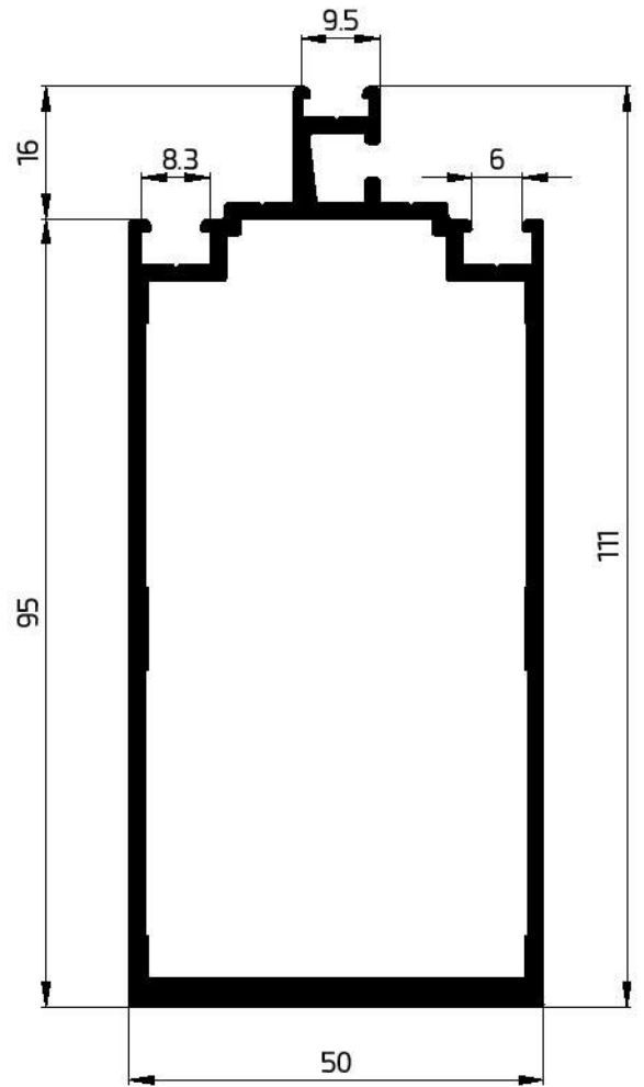
55033 CW-TRANSOM 50X95 1995 GR/M WT-2.0 mm
