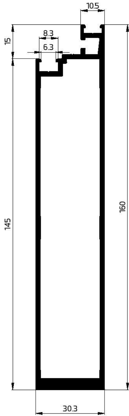
55045 CW-END TRANSOM 30X145 2407.47 GR/M WT-2.15 mm
