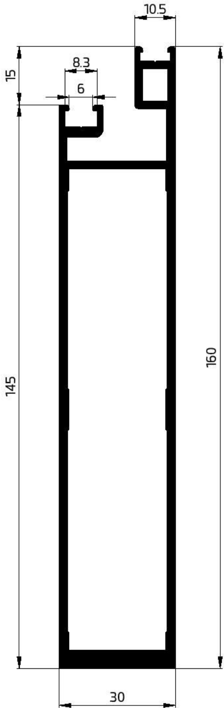
53002 CW-END MULLION 30X145 2550.88 GR/M WT-2.2 mm
