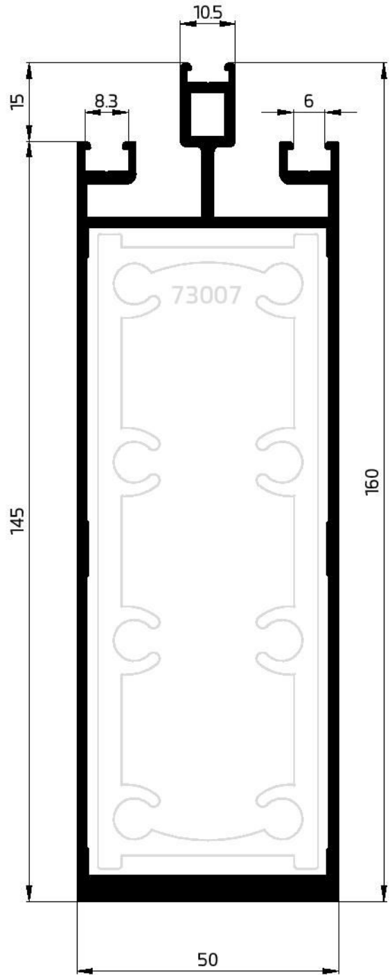
52027 CW-MULLION 50X145 3000 GR/M WT-2 mm
