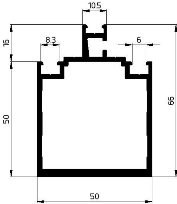
55047 CW-TRANSOM 50X50 1500.47 GR/M WT-2.15 mm
