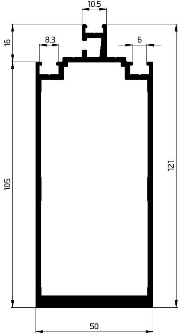
55028 CW-TRANSOM 50X105 2360.61GR/M WT-2.15 mm
