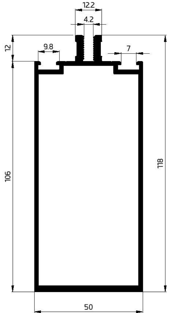
55011 CW-MULLION/TRANSOM 50X106 2044.81GR/M WT-2mm
