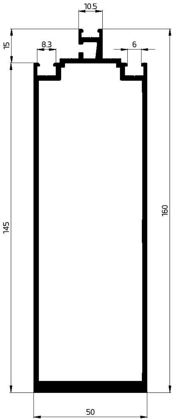
55044 CW-TRANSOM 50X145 2816.52 GR/M WT-2.15 mm
