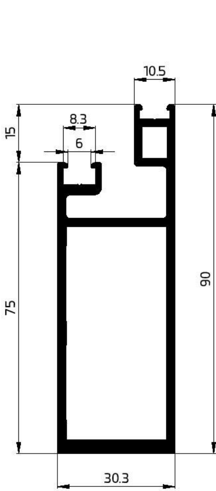
55025 CW-END MULLION 30X75 1605.28 GR/M WT-2.15 mm
