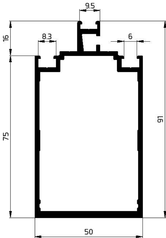
55032 CW-TRANSOM 50X75 1715 GR/M W T-2.0 mm
