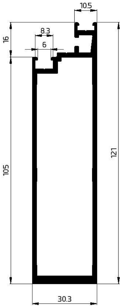
55024 CW-END TRANSOM 30X105 1856.76 GR/M WT-2.15 mm
