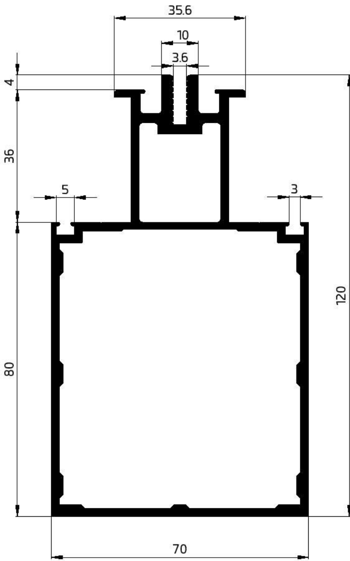
55503 CW-MULLION/TRANSOM 70X80 2812.91GR/M WT-2.2 mm
