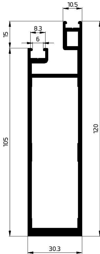
55049 CW-END MULLION 30X105 2048.57 GR/M WT-2.2 mm
