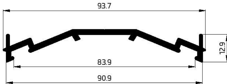
55052 CW-PRESSURE PLATE 785.98 GR/M WT-2.35 mm
