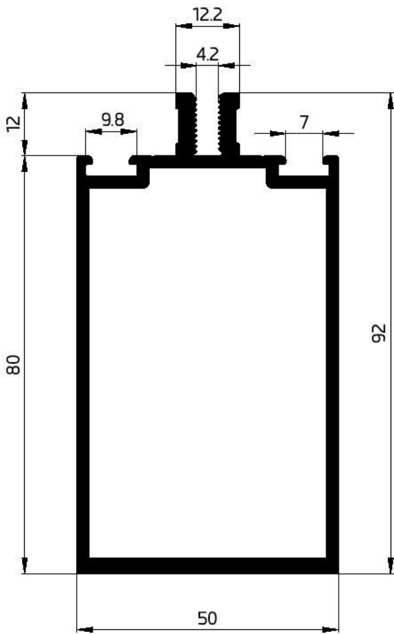
55012 CW-MULLION/TRANSOM 50X80 1910 GR/M WT-2.28mm
