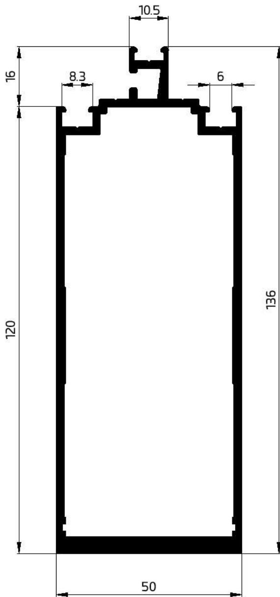
55043 CW-TRANSOM 50X120 2543.66 GR/M WT-2.2 mm
