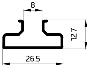
44007 PLYWOOD PROFILE 8 177.11 GR/M W.T- 1mm 42013 PLYWOOD PROFILE 8 158.15 GR/M W.T- 0.9mm
