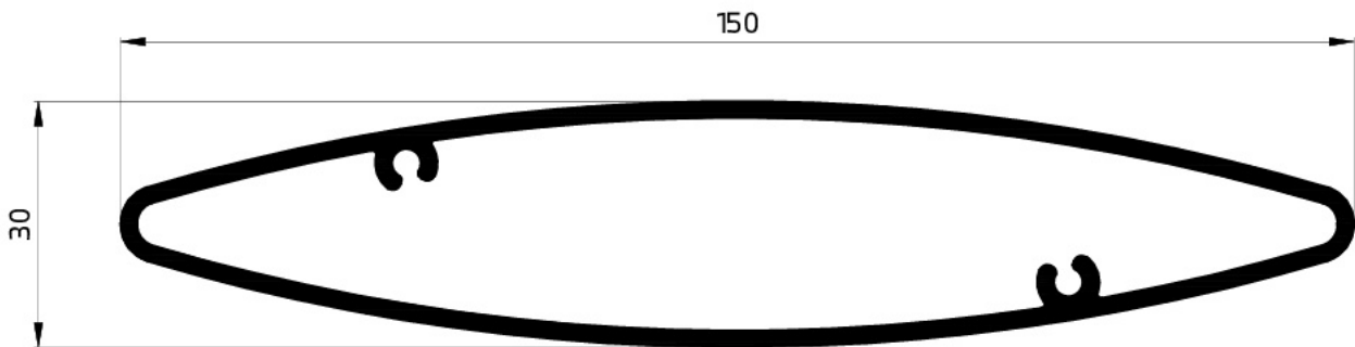
71001 OVAL LOUVER 1792.13 GR/M W.T-2mm
