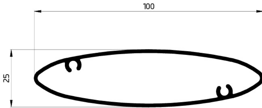
71012 OVAL LOUVER 928.58 GR/M W.T-15mm
