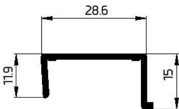
10262 SIGN BOARD COVER 2017 GR/M W.T - 1.35 mm
