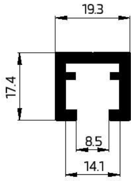
10100 BACK CHANNEL 404.15 GR/M W.T - 2.6 mm
