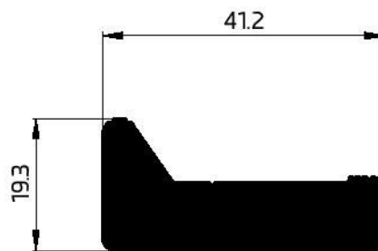
10327 PLANKING CLIP 1292.93 GR/M W.T - 10 mm
