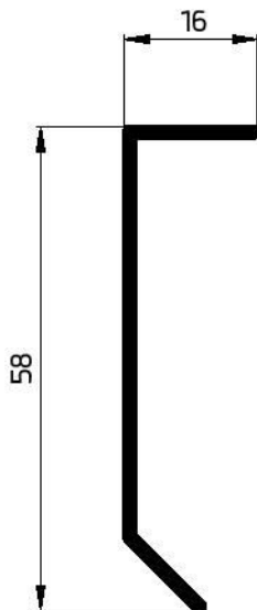
10031 SIGNAGE FRAME COVER 287.94 GR/M W.T - 1.4 mm
