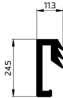
10030 SIGNAGE FRAME LOCK 305.33 GR/M W.T - 2.3 mm
