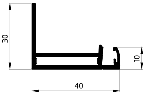
10129 SOLAR PANEL FRAME 522.77 GR/M W.T-1.7mm
