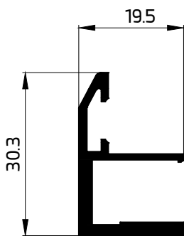
10111 PANEL END CLAMP FOR 10112 354.15 GR/M
