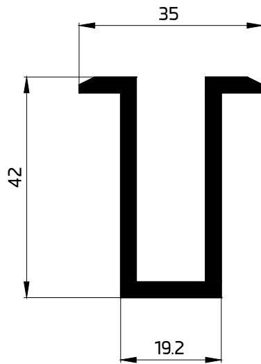
10110 SOLAR PANEL MIDDLE CLAMP 906.49 GR/M W.T - 3 mm
