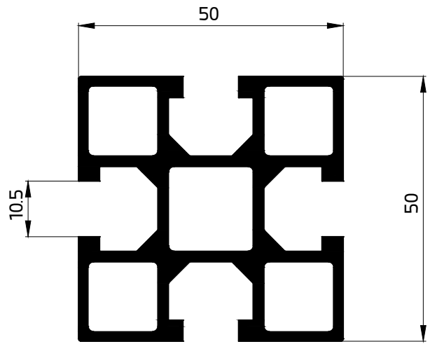
10123 SOLAR PANEL FRAME 2013.84 GR/M W.T - 2 mm
