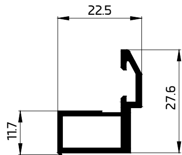
10112 PANEL END CLAMP FOR 10111 326.54 GR/M
