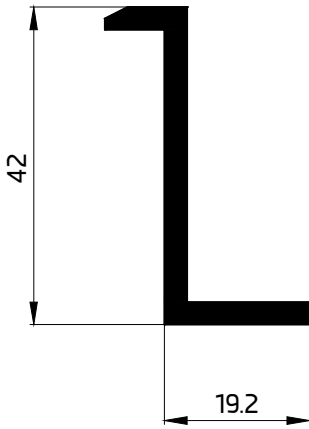
10115 SOLAR PANEL END CLAMP 531.29 GR/M W.T - 3 mm
