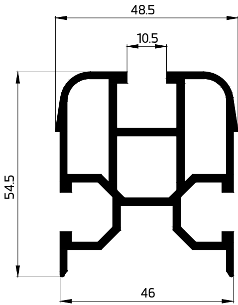
10108 SOLAR PANEL FRAME 1526.58 GR/M W.T - 2 mm
