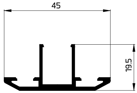
10114 PANEL MIDDLE CLAMP FOR 10113 386.36 GR/M
