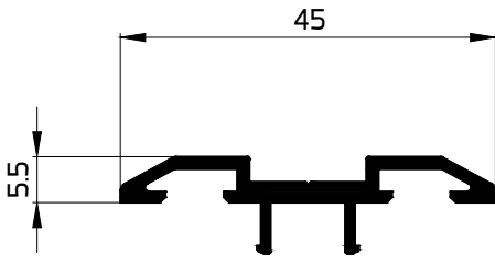
10113 PANEL MIDDLE CLAMP FOR 10114 341.19 GR/M
