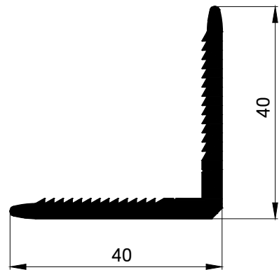
10130 FRAME CONNECTOR FOR 10129 672.08 GR/M W.T - 3.8 mm
